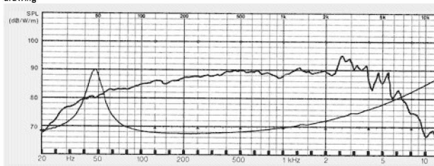
frequency response
