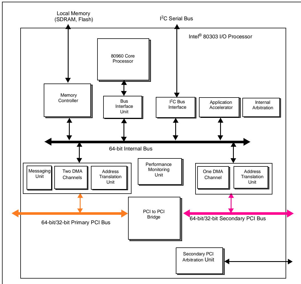
Figure 1. Intel® 80303 I/O Processor Functional Block Diagram
