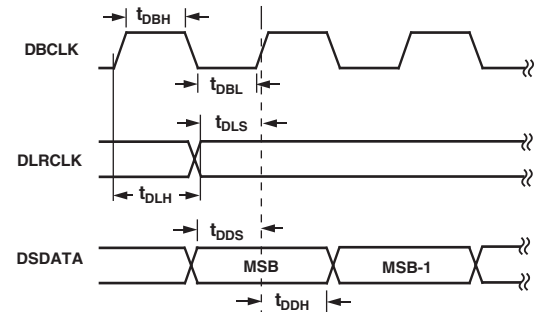
Figure 10. DAC Packed Mode Timing
