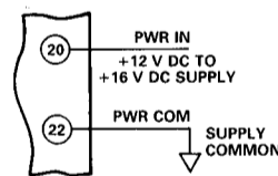
Figure 15. Powering the AD203SN
