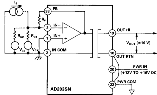
Figure 19. Input Configuration for Summing or Current Input
