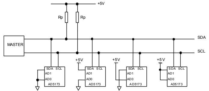
Figure 18. Multiple AD5173 Devices on One I 2 C Bus
