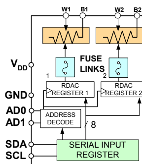
Figure 2. AD5173
