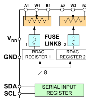
Figure 1. AD5172
