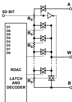
Figure 17. AD5172/73 Equivalent RDAC Circuit
