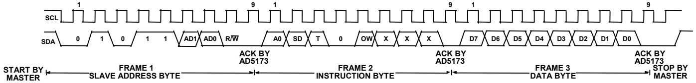
Figure 14. Writing to the RDAC Register – AD5173
