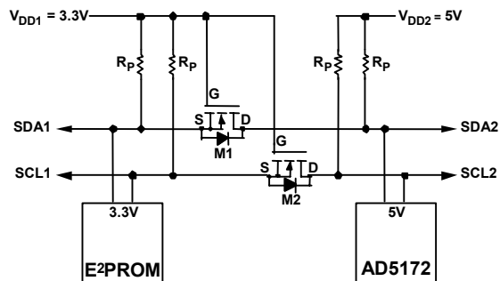
Figure 19. Level Shifting for Operation at Different Potentials
