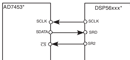
Figure 17. Interfacing to the DSP56xx
