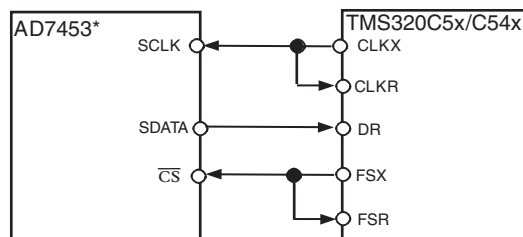
Figure 15. Interfacing to the TMS320C5x/C54x
