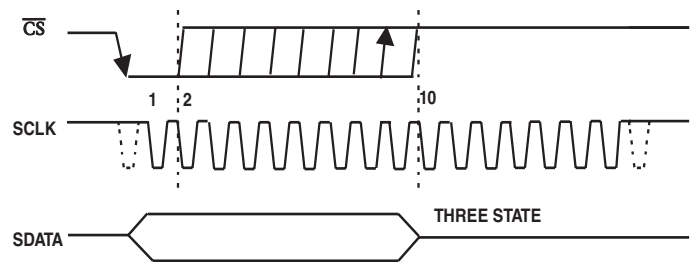
Figure 12. Entering Power Down Mode
