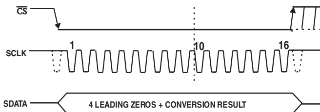
Figure 11. Normal Mode Operation
