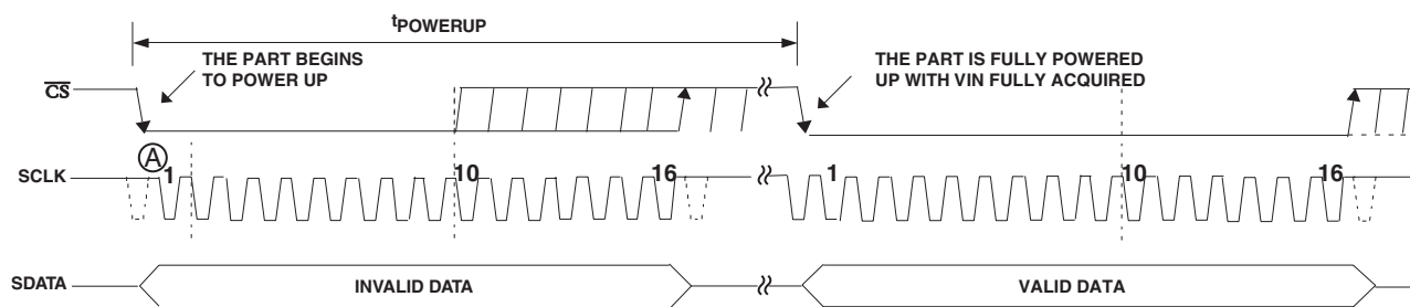
Figure 13. Exiting Power Down Mode
