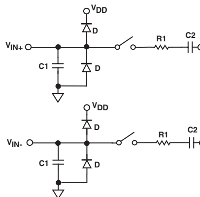
Figure 7. Equivalent Analog Input Circuit. Conversion Phase - Switches Open Track Phase - Switches Closed
