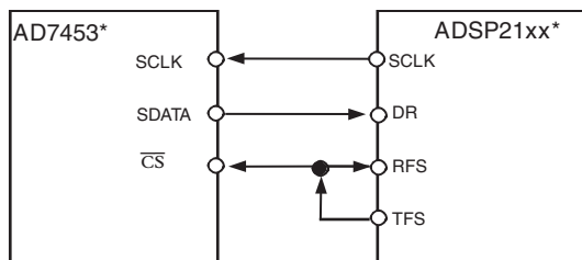
Figure 14. Interfacing to the ADSP 21xx
