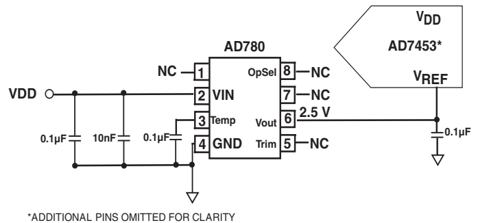
Figure 10. Typical V_{REF} Connection Diagram for V_{DD} = 5 V
