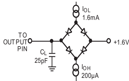
Figure 2. Load Circuit for Digital Output Timing Specifications
