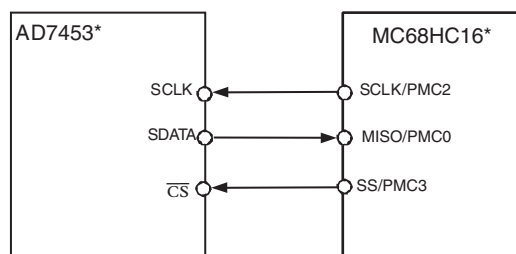
Figure 16. Interfacing to the MC68HC16
