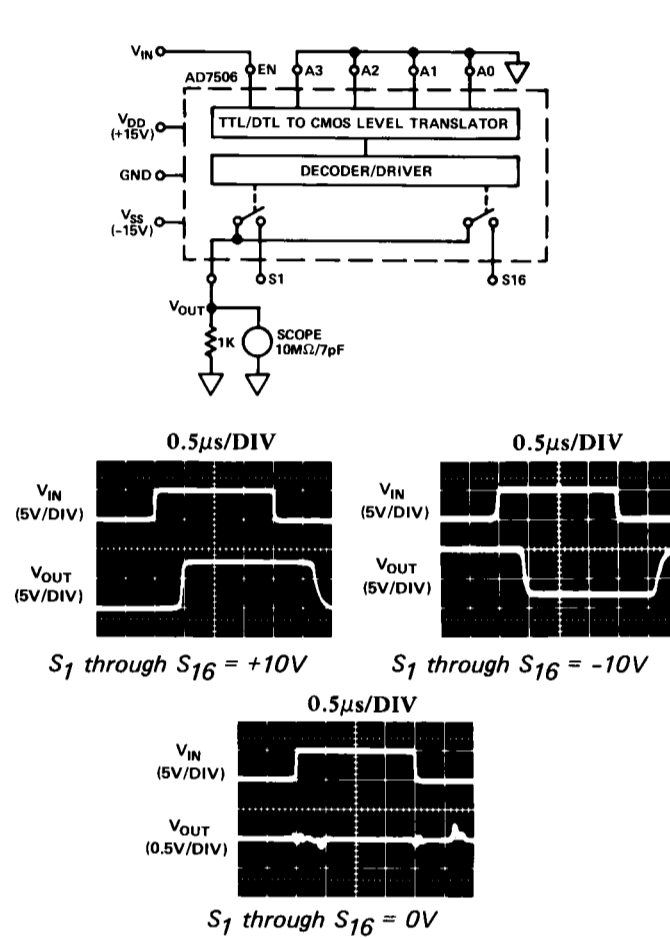
TEST CIRCUIT 2
