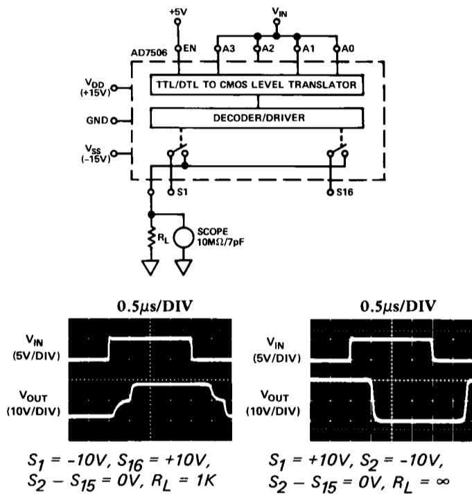
TEST CIRCUIT 1
