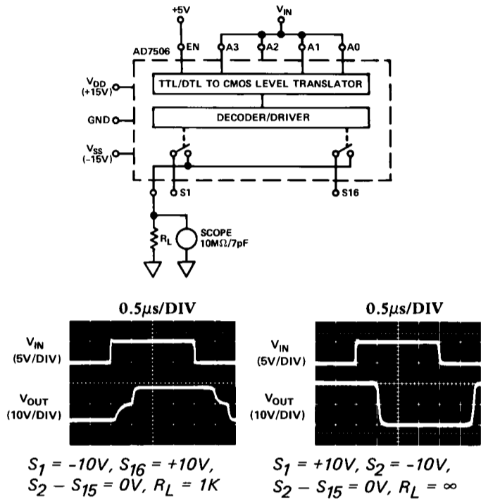
TEST CIRCUIT 1
