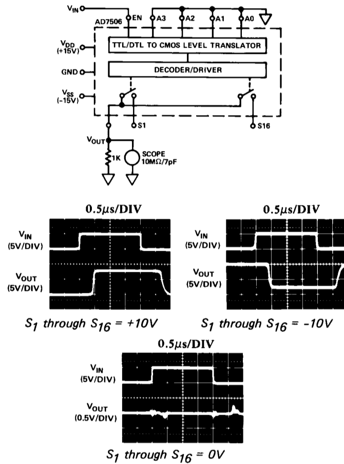
TEST CIRCUIT 2
