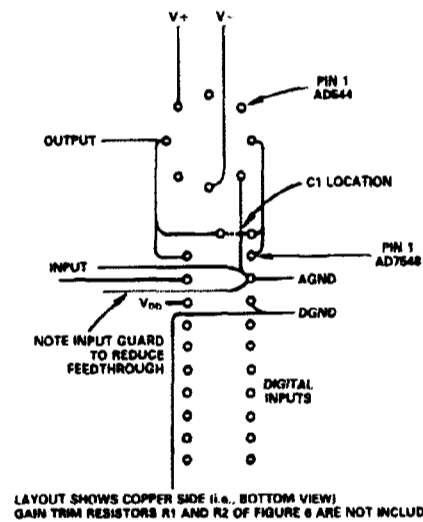
Figure 9. Suggested Layout for AD7548 and Op Amp
