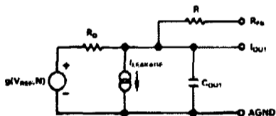
Figure 3. AD7548 Equivalent Analog Output Circuit
