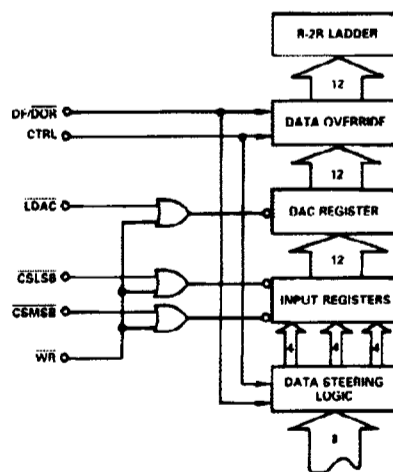
Figure 1b. Simplified AD7548 Input Control Structure
