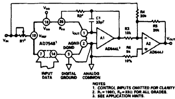
Figure 7. Bipolar Operation (Offset Binary Coding)
