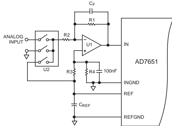
Figure 23. Using the AD7651 in 16-Bit Bipolar and/or Wider Input Ranges
