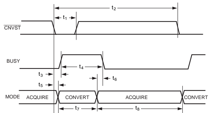
Figure 11. Basic Conversion Timing
