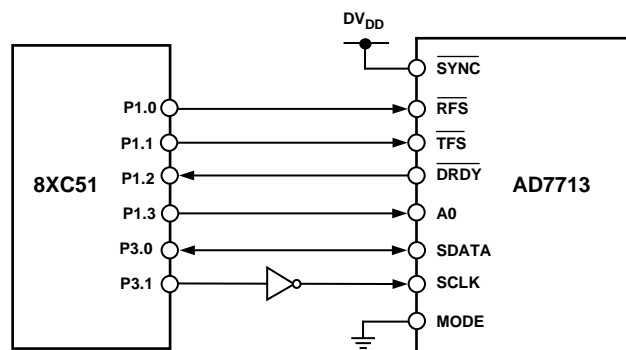
Figure 17. AD7713 to 8XC51 Interface
