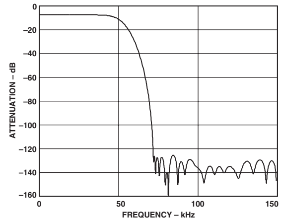
Figure 21. Default Filter Response for CLKIN = 9.6 MHz
