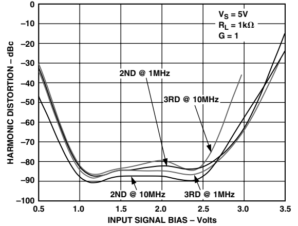
Figure 12. Harmonic Distortion for a 1 V p-p Signal vs. Input Signal DC Bias
