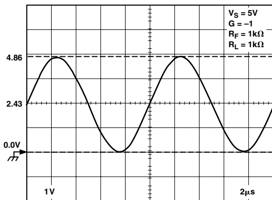
Figure 35. Output Swing
