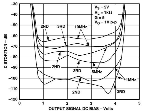
Figure 14. Harmonic Distortion vs. Output Signal DC Bias
