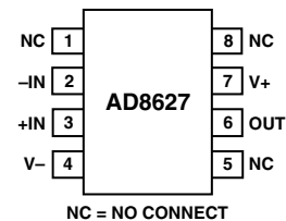
8-Lead SOIC (RN Suffix)
