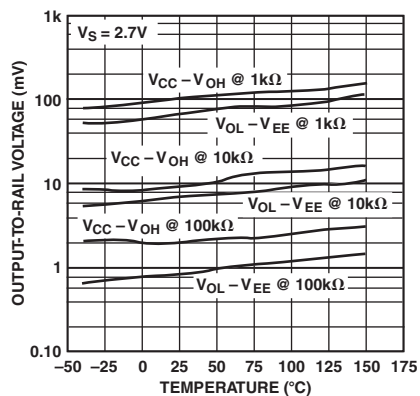
TPC 43. Output-to-Rail Voltage vs. Temperature
