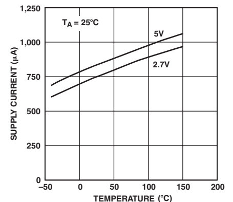
TPC 9. Supply Current vs. Temperature
