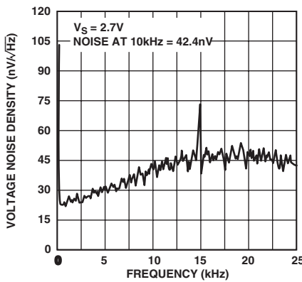
TPC 35. Voltage Noise Density at 2.7 V from 0 Hz to 25 kHz
