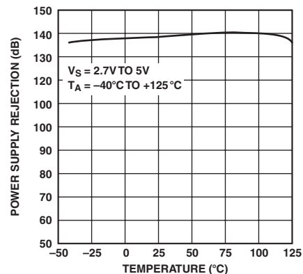
TPC 39. Power Supply Rejection vs. Temperature
