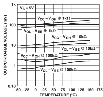
TPC 42. Output-to-Rail Voltage vs. Temperature
