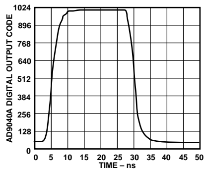
Figure 14. Transient Response
