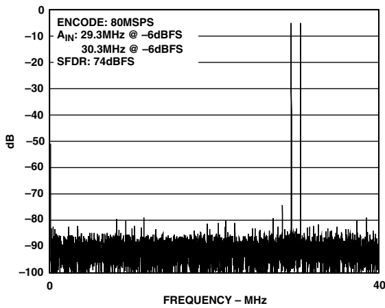
TPC 8. Two-Tone Intermodulation Distortion (29.3 MHz, 30.3 MHz; 1 V p-p, f_S = 80 MSPS)
