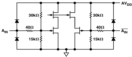
Figure 2. Analog Input Stage
