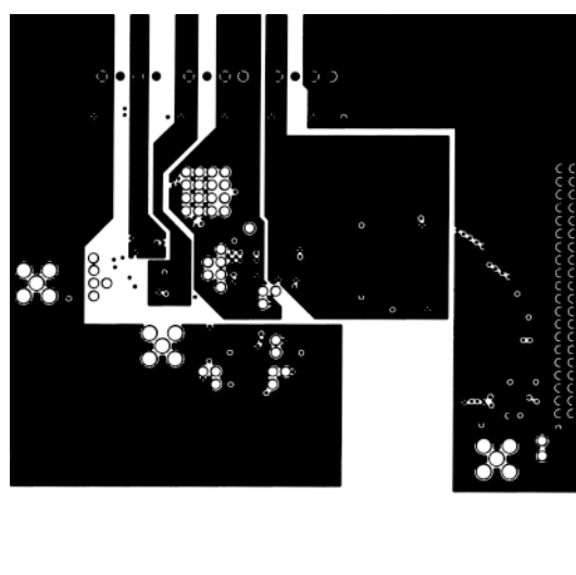
Figure 16. PCB Power Layers—Layers 3 and 4
