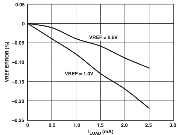
Figure 14. VREF Accuracy vs. Load
