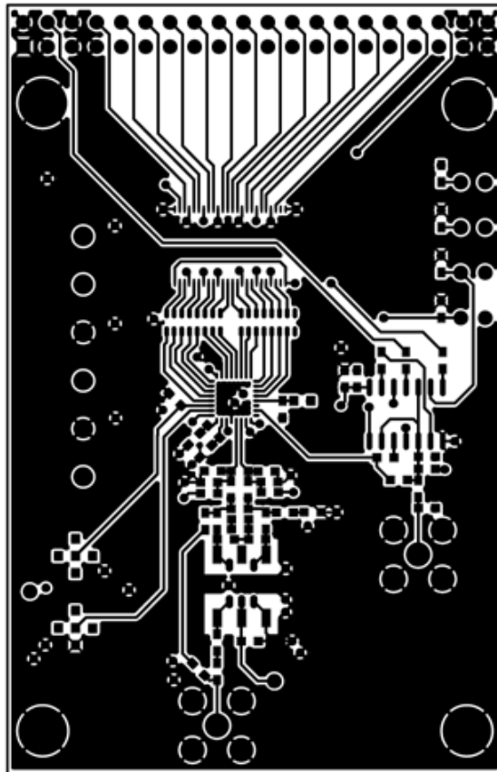
Figure 20. LFCSP Evaluation Board Layout, Primary Side
