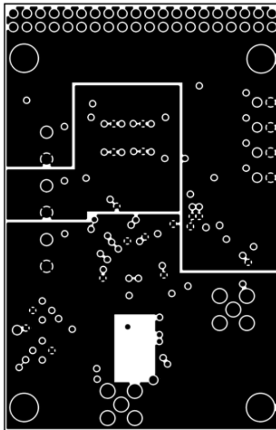
Figure 23. LFCSP Evaluation Board Layout, Power Plane
