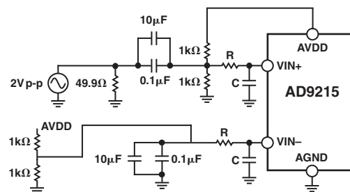
Figure 10. Single-Ended Input Configuration
