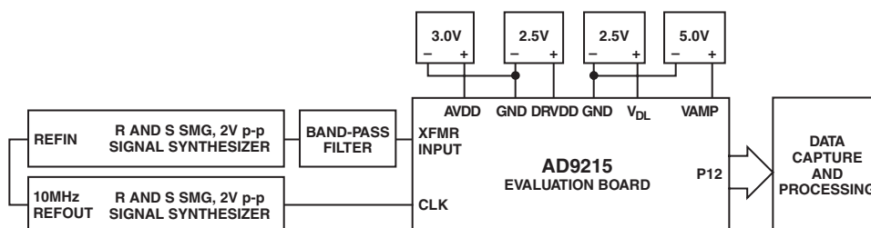
Figure 16. Evaluation Board Connections
