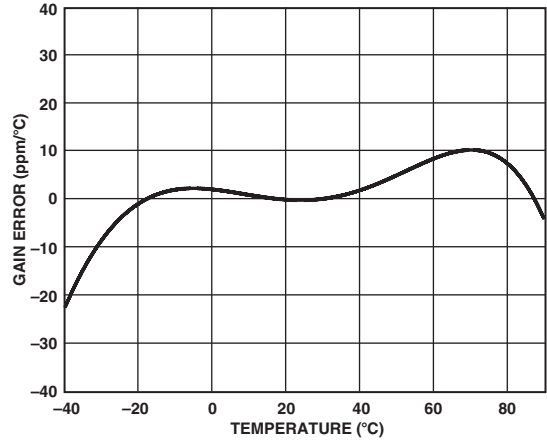
TPC 17. Gain vs. Temperature External 1 V Reference
