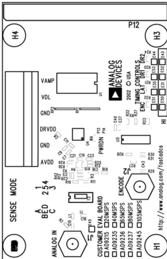
Figure 24. LFCSP Evaluation Board Layout, Primary Silkscreen
