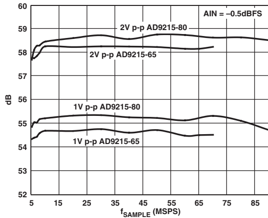
TPC 14. SINAD vs. f_{SAMPLE} , f_{IN} = 40.9 MHz
