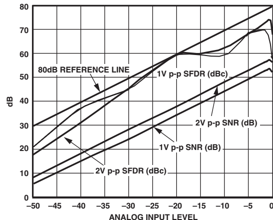
TPC 6. AD9215-80 SNR/SFDR vs. Analog Input Drive Level, f_{SAMPLE} = 80 MSPS, f_{IN} = 39.1 MHz
