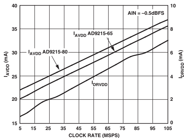
Figure 11. Supply Current vs. f_{\text{SAMPLE}} for f_{\text{IN}} = 10.3 \text{ MHz}
