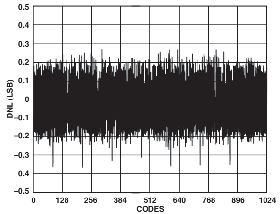
TPC 18. AD9215-80 Typical DNL, f_{SAMPLE} = 80 MSPS, f_{IN} = 2.3 MHz
