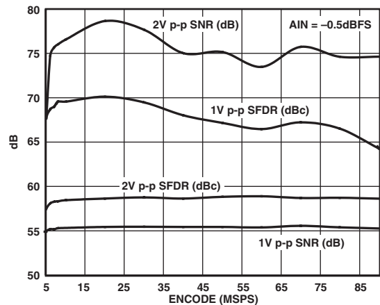
TPC 4. AD9215-80 SNR/SFDR vs. f_{SAMPLE} , f_{IN} = 10.3 MHz
