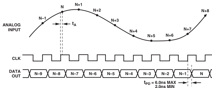
Figure 1. Timing Diagram
