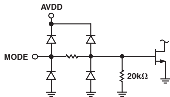
Figure 3. Equivalent MODE Input Circuit
