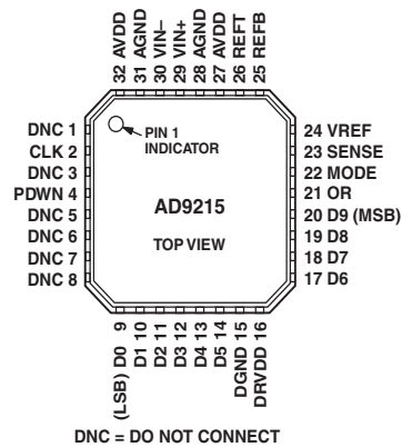
LFCSP (CP-32)
