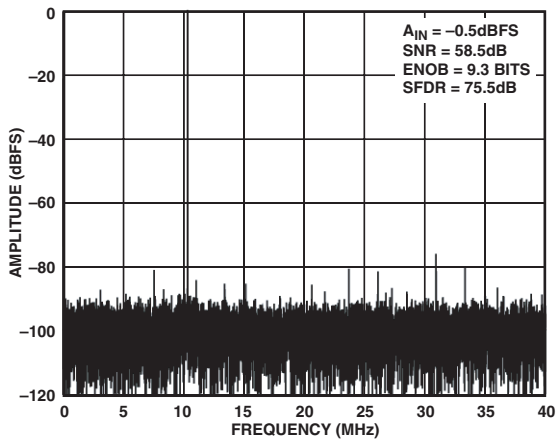
TPC 1. Single-Tone 32k FFT with f_{IN} = 10.3 MHz f_{SAMPLE} = 80 MSPS
