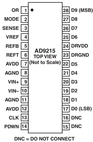
TSSOP (RU-28)
