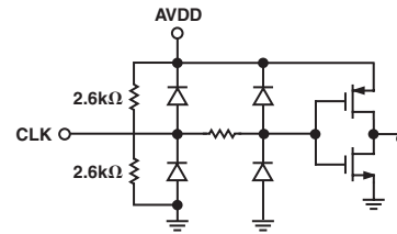
Figure 5. Equivalent Digital Input Circuit
