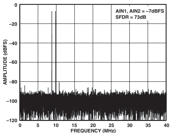
TPC 10. Two-Tone 32k FFT with f_{IN1} = 70.3 MHz, and f_{IN2} = 71.3 MHz, f_{SAMPLE} = 80 MSPS
