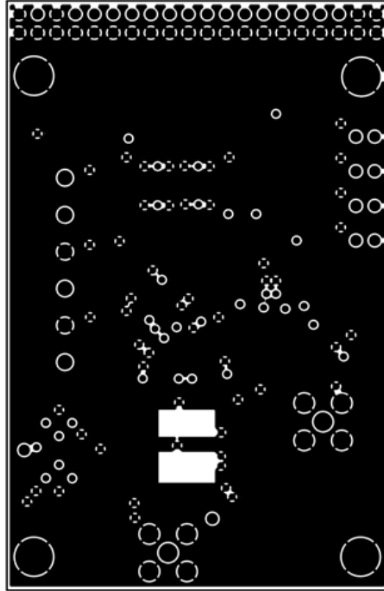
Figure 22. LFCSP Evaluation Board Layout, Ground Plane
