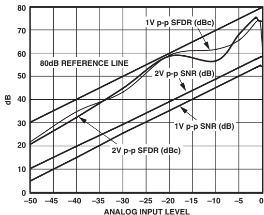
TPC 7. AD9215-65 SNR/SFDR vs. Analog Input Drive Level, f_{SAMPLE} = 65 MSPS, f_{IN} = 30.3 MHz
