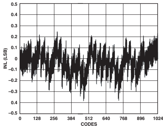
TPC 19. AD9215-80 Typical INL, f_{\text{SAMPLE}} = 80 \text{ MSPS} , f_{\text{IN}} = 2.3 \text{ MHz}
