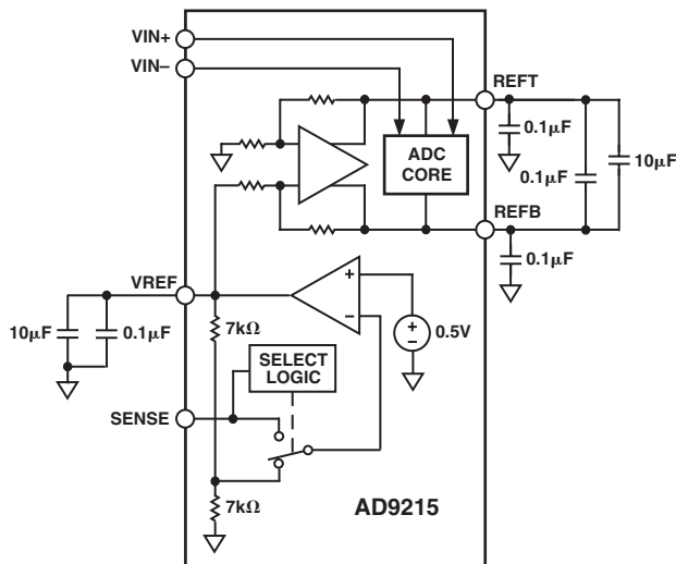
Figure 12. Internal Reference Configuration
