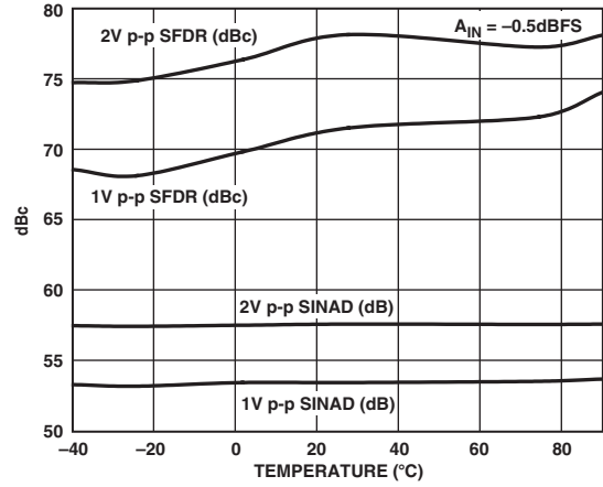
TPC 16. SINAD, SFDR vs. Temperature, f_{IN} = 39 MHz
