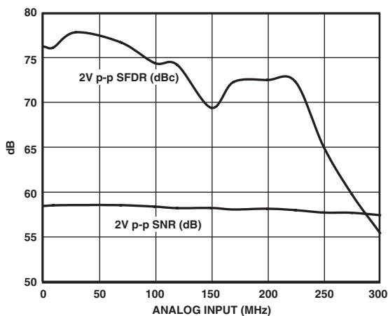
TPC 9. AD9215-65 SNR/SFDR vs. f_{IN} , A_{IN} = -0.5 dBFS, f_{SAMPLE} = 65 MSPS
