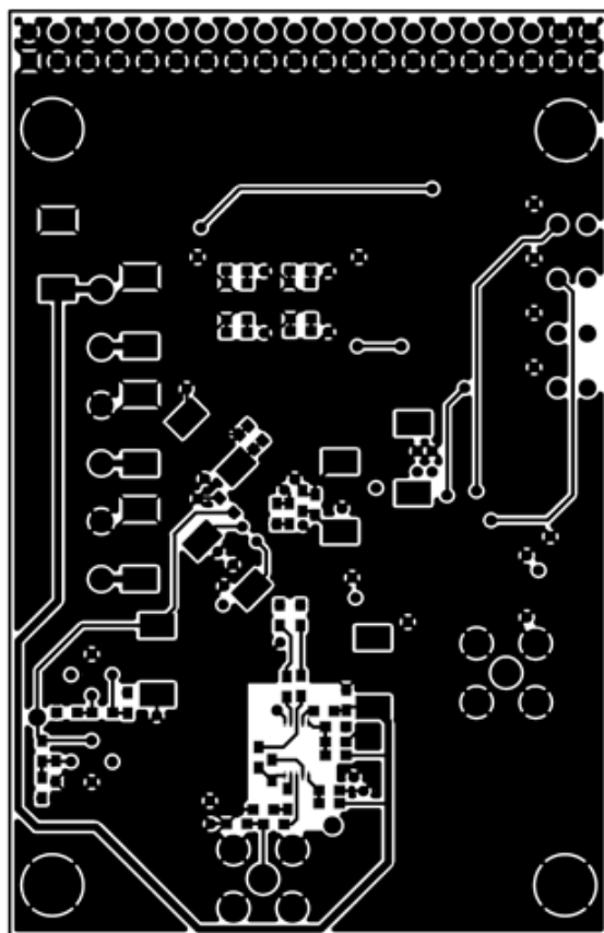
Figure 21. LFCSP Evaluation Board Layout, Secondary Side
