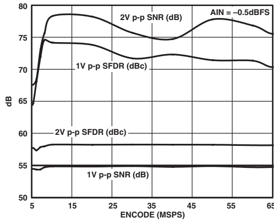
TPC 5. AD9215-65 SNR/SFDR vs. f_{SAMPLE} , f_{IN} = 10.3 MHz
