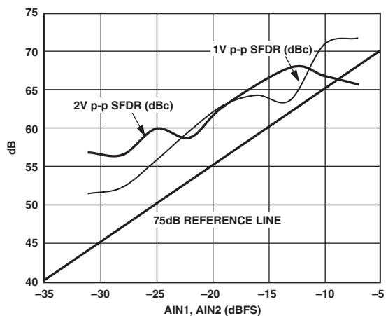
TPC 12. AD9215-80 Two-Tone SFDR vs. A_{IN} , f_{IN1} = 69.3 MHz, and f_{IN2} = 70.3 MHz, f_{SAMPLE} = 80 MSPS
