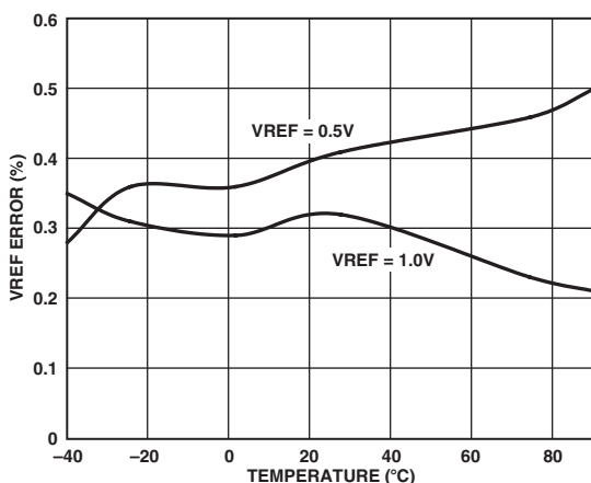
Figure 15. Typical VREF Drift
