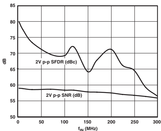
TPC 8. AD9215-80 SNR/SFDR vs. f_{IN} , A_{IN} = -0.5 dBFS, f_{SAMPLE} = 80 MSPS
