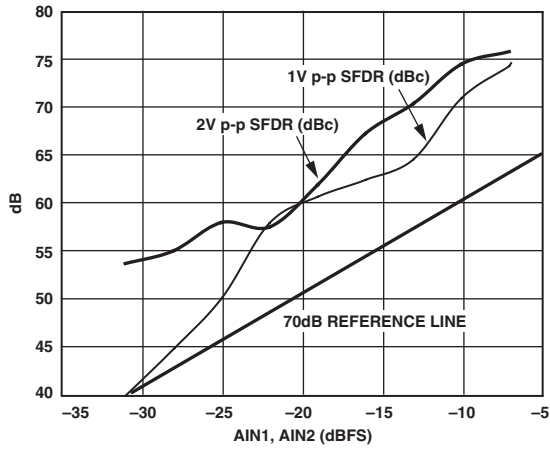
TPC 13. AD9215-80 Two-Tone SFDR vs. A_{IN} , f_{IN1} = 100.3 MHz, and f_{IN2} = 101.3 MHz, f_{SAMPLE} = 80 MSPS
