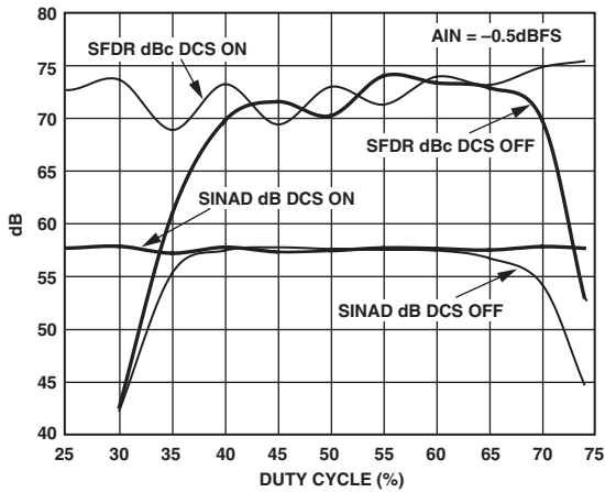
TPC 15. SINAD, SFDR vs. Clock Duty Cycle, f_{SAMPLE} = 80 MSPS, f_{IN} = 40.9 MHz
