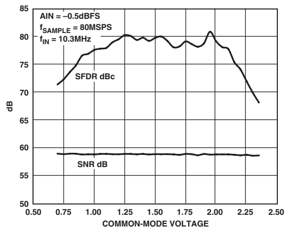
Figure 7. AD9215-80 SNR, SFDR vs. Common-Mode Voltage
