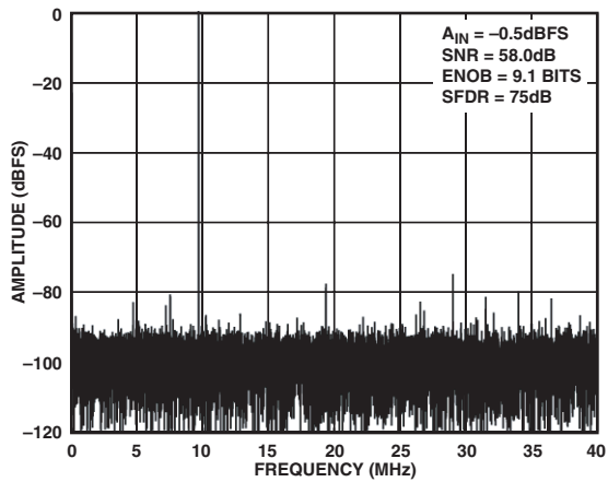
TPC 2. Single-Tone 32k FFT with f_{IN} = 70.3 MHz, f_{SAMPLE} = 80 MSPS
