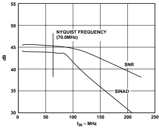
Figure 29. SNR vs. f_{IN} : f_S = 140 MSPS
