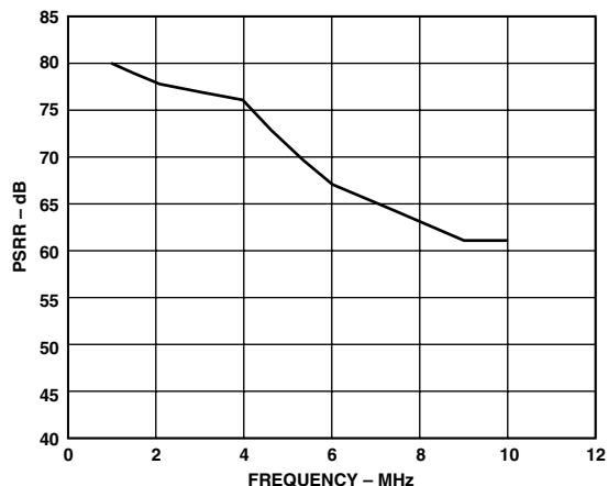
Figure 25. Power Supply Rejection Ratio
