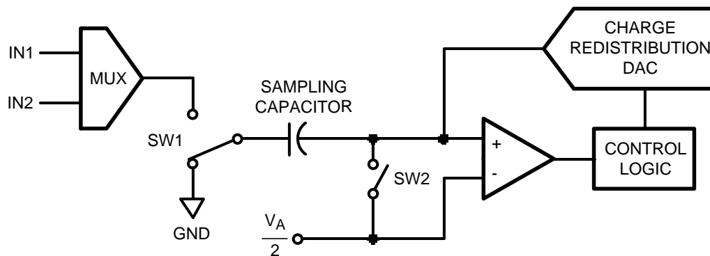
Figure 49. ADC082S101 in Hold Mode
