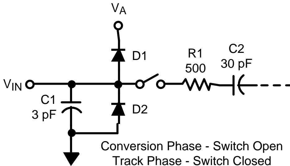
Figure 52. Equivalent Input Circuit
