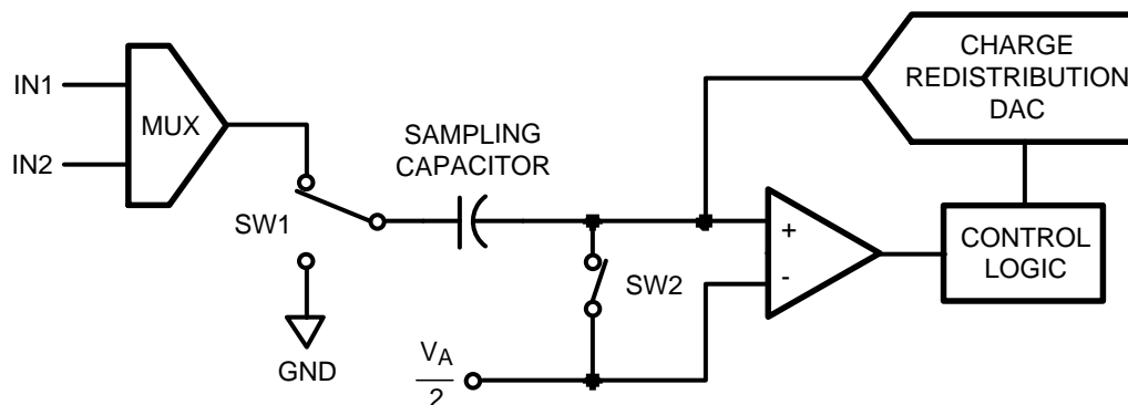
Figure 48. ADC082S101 in Track Mode
