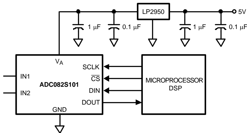
Figure 51. Typical Application Circuit
