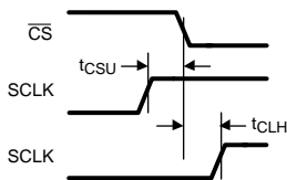
Figure 5. SCLK and CS Timing Parameters
