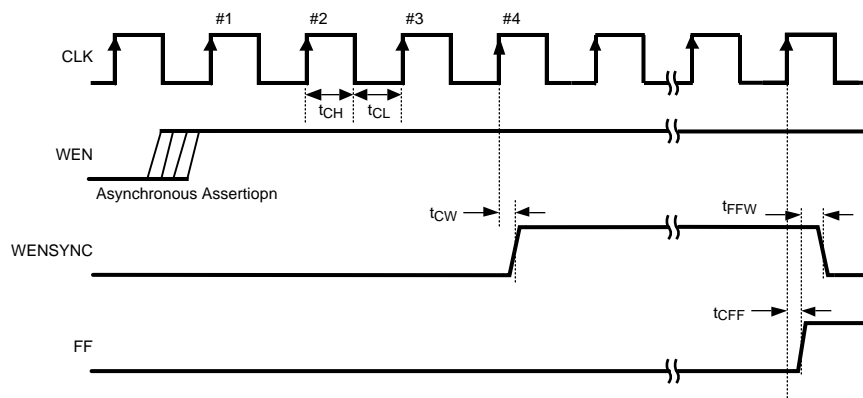
Figure 3. ADC08B200 Buffer Write Timing
