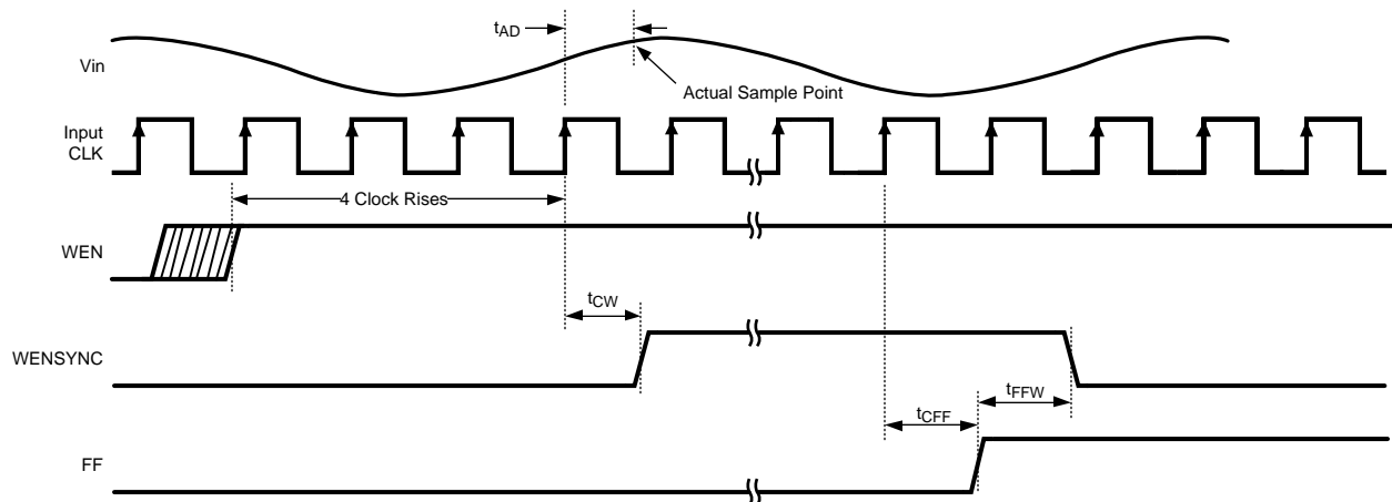
Figure 2. ADC08B200 Capture and Write Enable Timing
