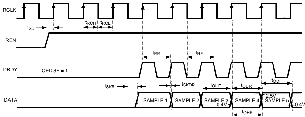
Figure 4. ADC08B200 Buffer Read Timing (OEDGE/TEN = 1)
