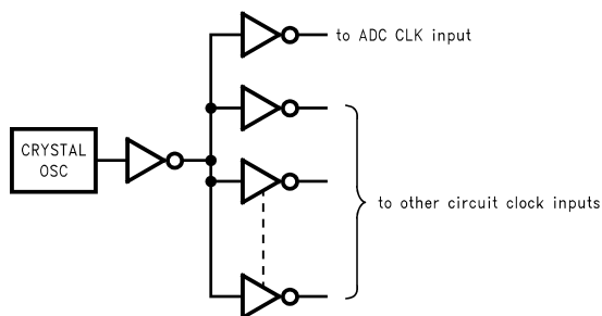
Figure 11. Isolating the ADC Clock from Digital Circuitry
