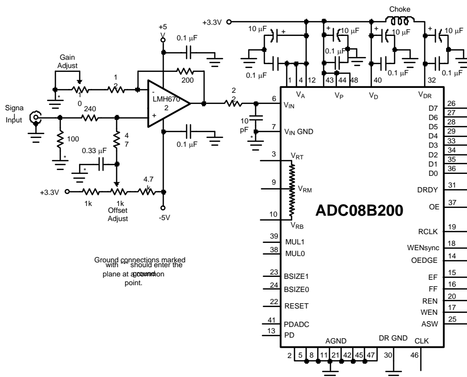
Figure 9. The input amplifier should incorporate some gain for best performance (see text).
