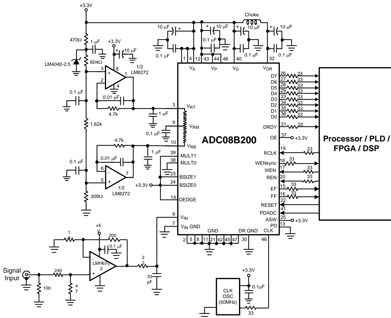
Figure 10. Example of a Typical Application.
