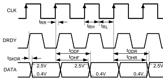
Figure 6. ADC08B200 Buffer Bypassed Timing
