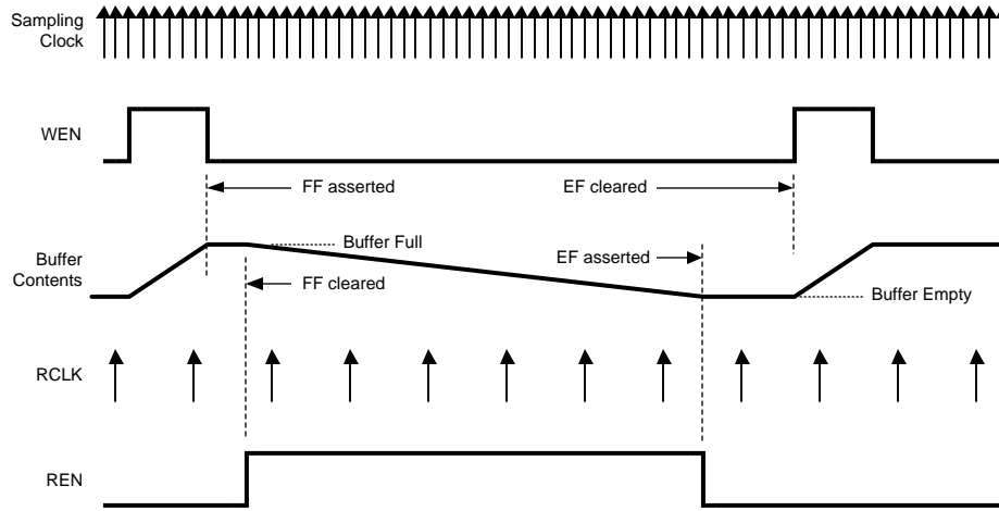
Figure 1. ADC08B200 Data Capture and Read Operation
