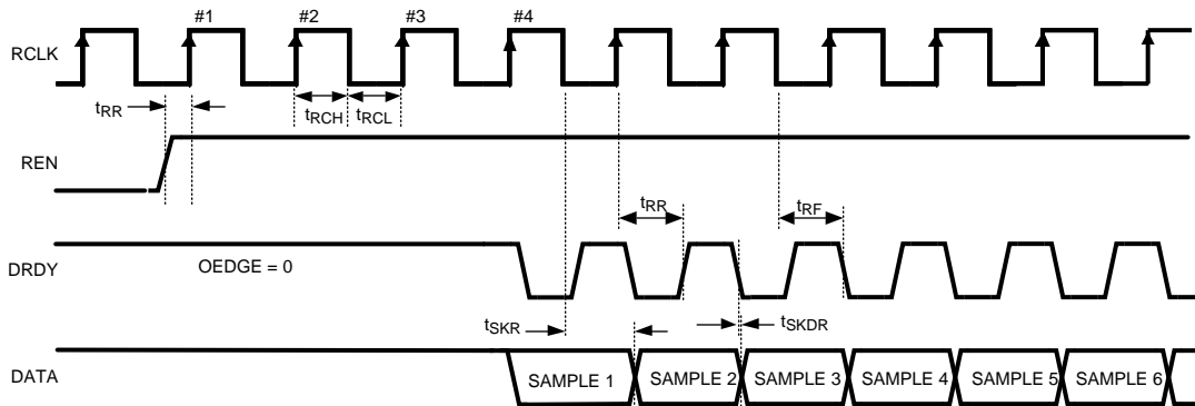
Figure 5. ADC08B200 Buffer Read Timing (OEDGE/TEN = 0)
