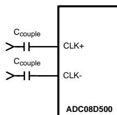
Figure 34. Differential (LVDS) Clock Connection
