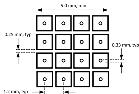
Figure 36. Recommended Package Land Pattern
