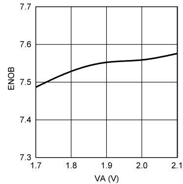
ENOB vs. SUPPLY VOLTAGE
