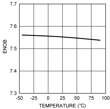
ENOB vs. TEMPERATURE
