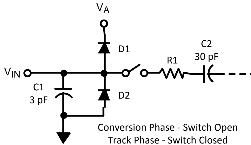
Figure 52. Equivalent Input Circuit
