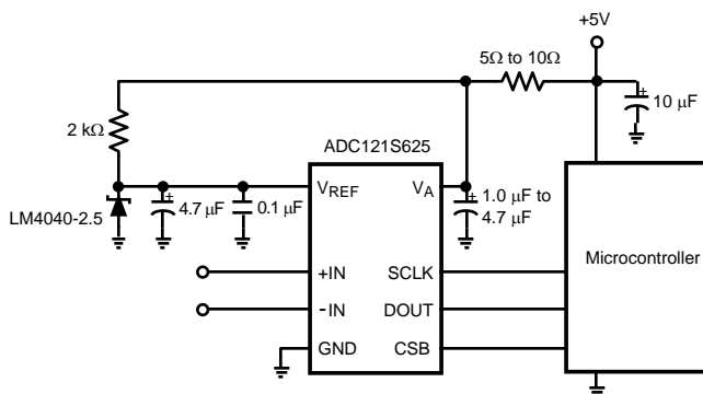
Figure 53. Low cost, low power Data Acquisition System
