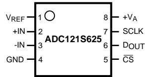
Figure 1. 8-Lead VSSOP See DGK Package
