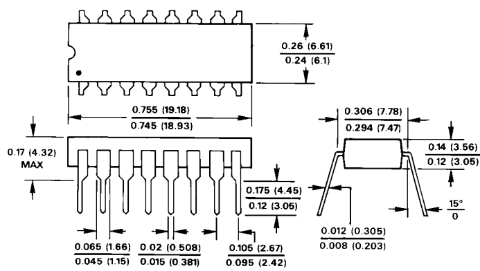
16-Pin Plastic (N-16)
