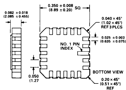
20-Terminal Leadless Ceramic Chip Carrier (E-20A)
