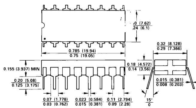
16-Pin Cerdip (Q-16)
