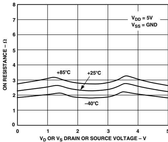
Figure 5. On Resistance as a Function of V_D ( V_S ) for Different Temperatures; V_{DD} = 5 V
