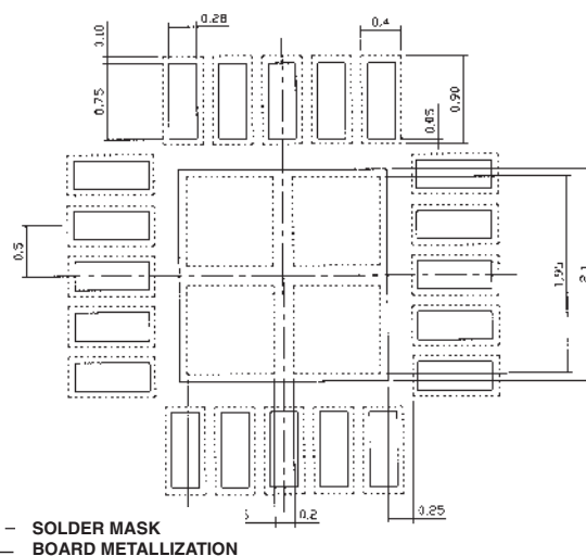
Figure 3. Suggested LFCSP 4 \times 4 20-Lead Land Pattern
