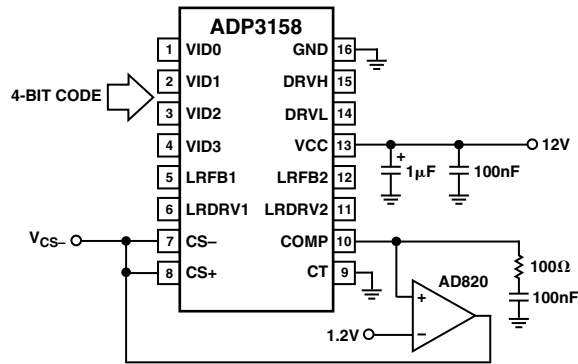
Figure 1. Closed Loop Output Voltage Accuracy Test Circuit
