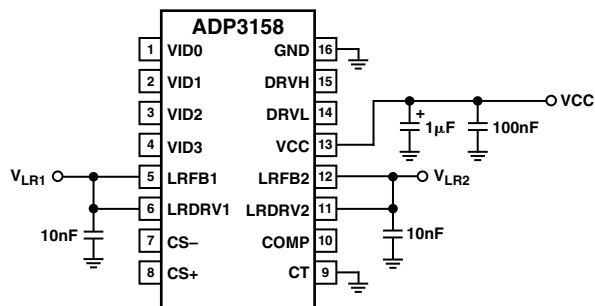
Figure 2. Linear Regulator Output Voltage Accuracy Test Circuit
