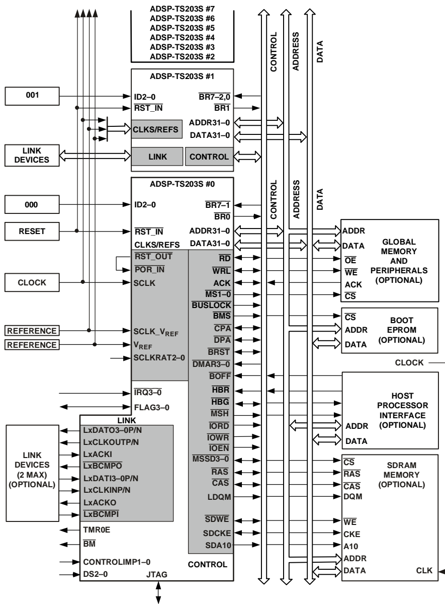
Figure 3. ADSP-TS203S Shared Memory Multiprocessing System
