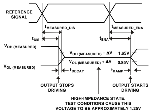
Figure 31. Output Enable/Disable
