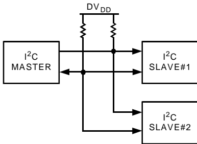
Figure 36. Typical I 2 C System
