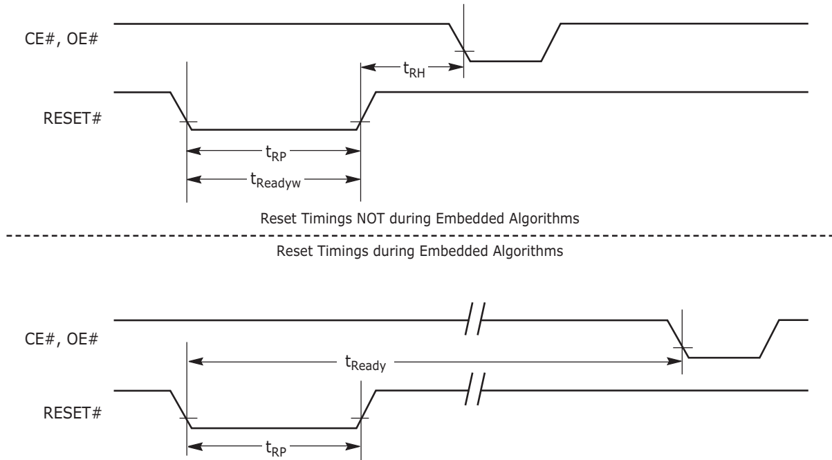
Figure 20. Reset Timings
