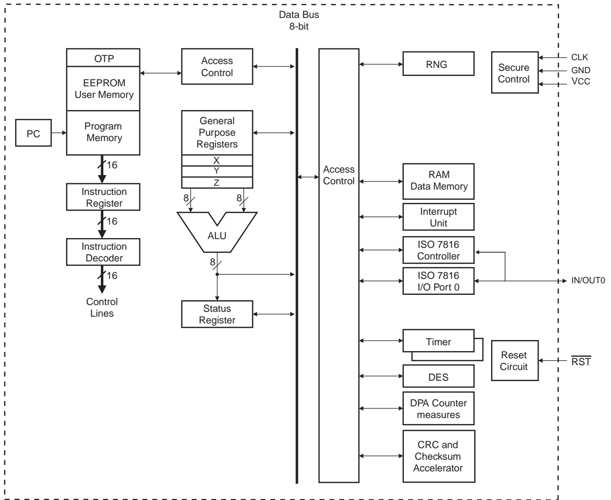
Figure 1. AT90SC6404R secureAVR RISC Architecture
