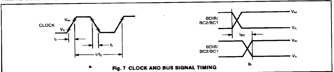
Fig. 7 CLOCK AND BUS SIGNAL TIMING
