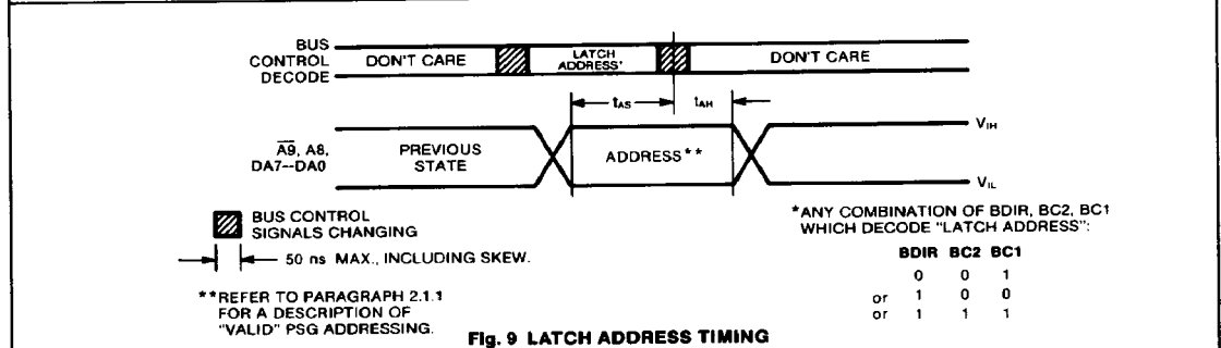
Fig. 9 LATCH ADDRESS TIMING
