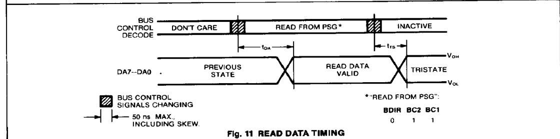
Fig. 11 READ DATA TIMING
