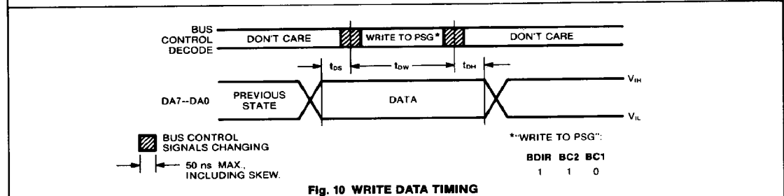
Fig. 10 WRITE DATA TIMING
