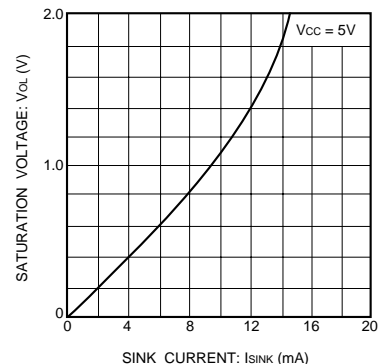
Fig. 3 Output voltage (logic 0 side) characteristics
