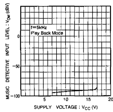
Fig. 19 Music detectable input level vs. supply voltage
