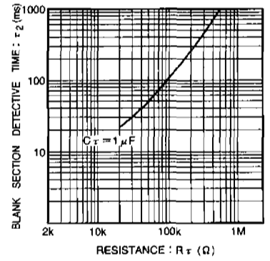
Fig. 22 Blank section detectable vs. time constant resistance
