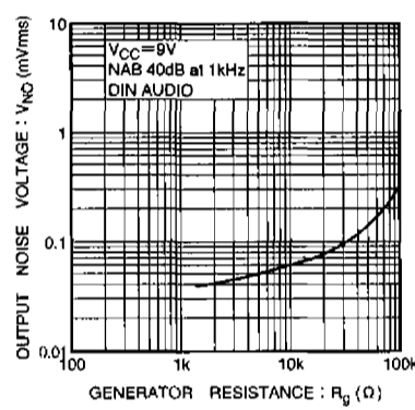
Fig. 18 Output noise voltage vs. generator resistance
