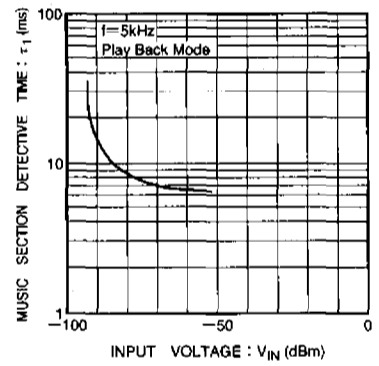
Fig. 20 Music section detectable time vs. input voltage
