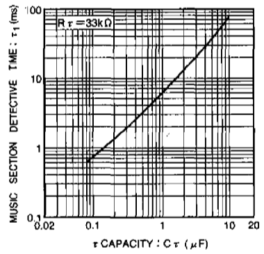
Fig. 21 Music section detectable time vs. time constant capacity
