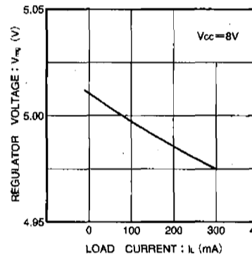
Fig. 11 Load current vs. regulator voltage
