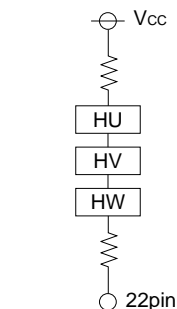
< Series connection >
