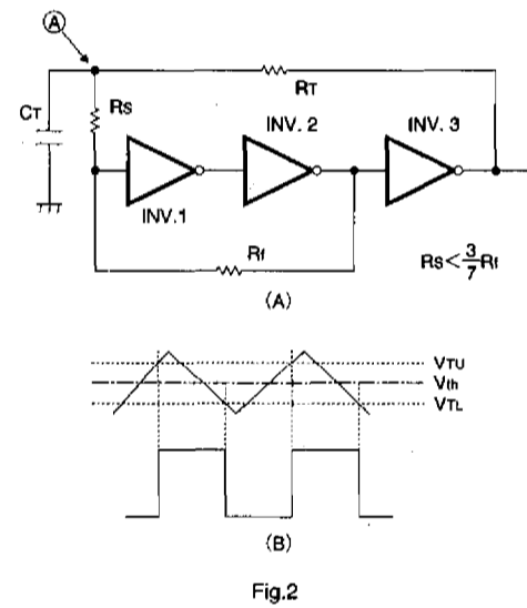
CR timers
