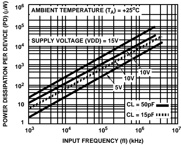
FIGURE 9. TYPICAL POWER DISSIPATION vs FREQUENCY
