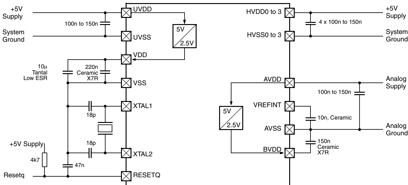
Fig. 2-3: CDC3207G-C: Recommended external supply and quartz connection.
