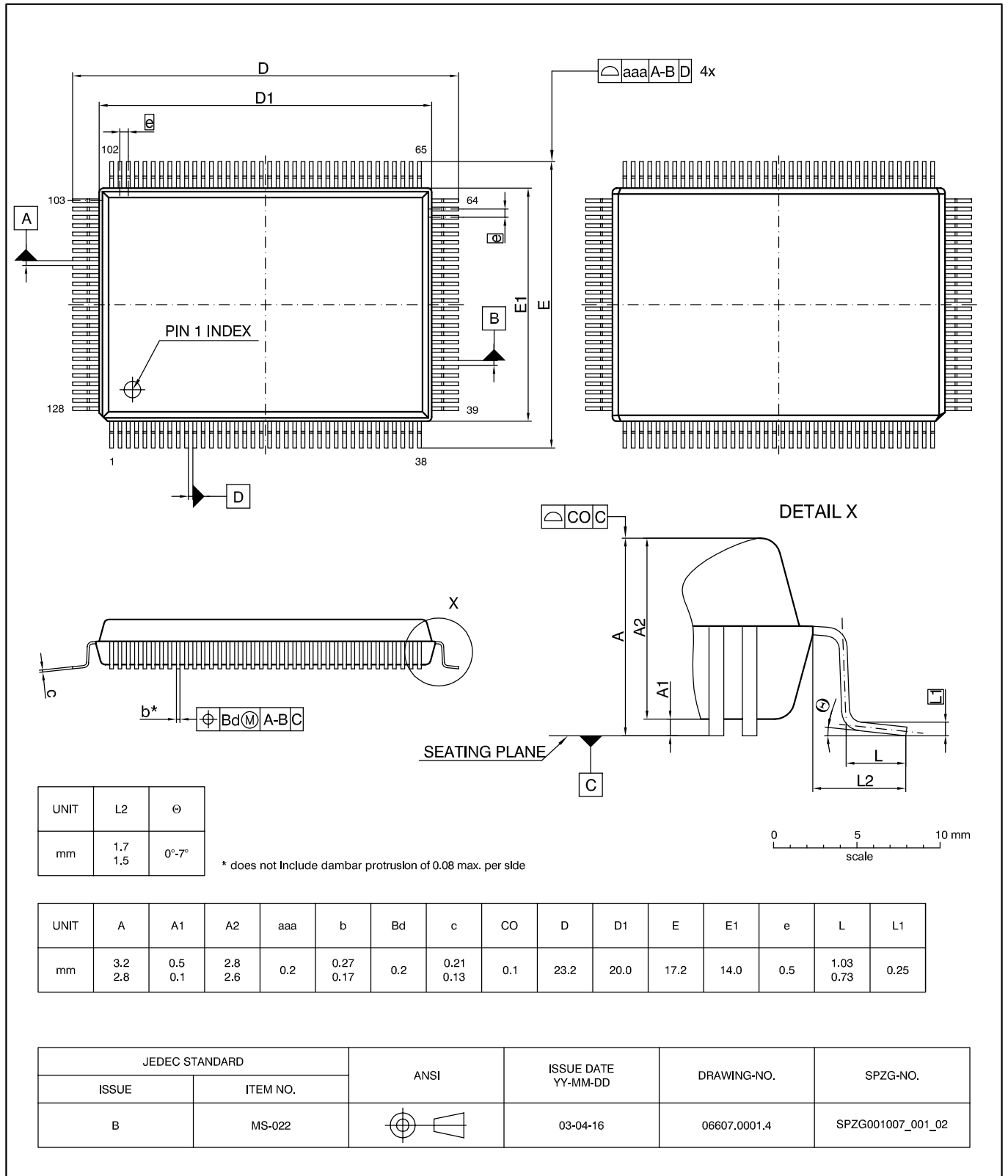
Fig. 2-1: PMQFP128-2: Plastic Metric Quad Flat Package, 128 leads, 14 × 20 × 2.7 mm 3 Ordering code: QK Weight approximately 1.8 g
