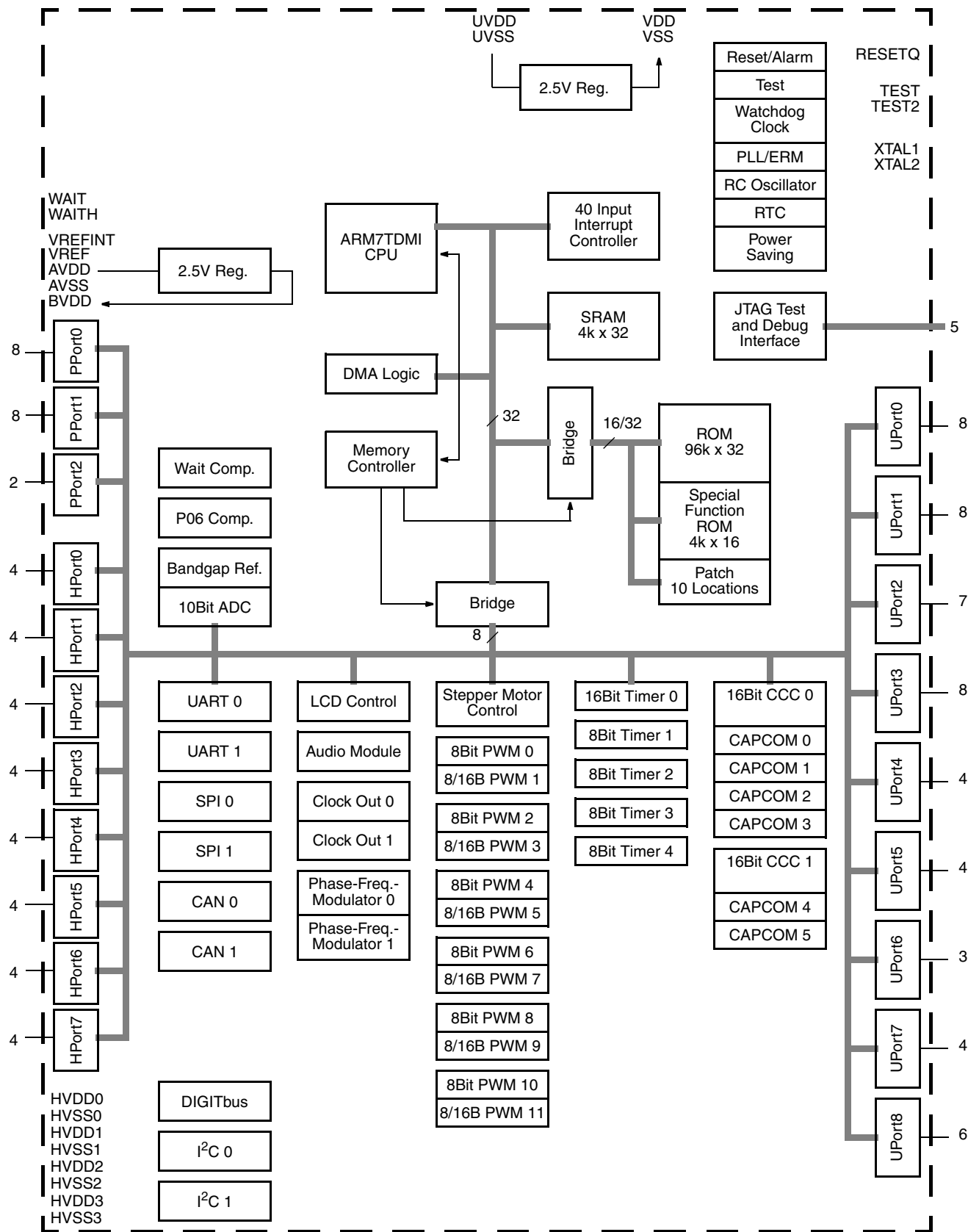
Fig. 1-1: CDC3272G-C block diagram
