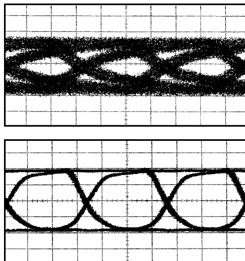
Figure 15. Before and After Equalization at 622 Mbps Through 50 Meters of Category 5 UTP
