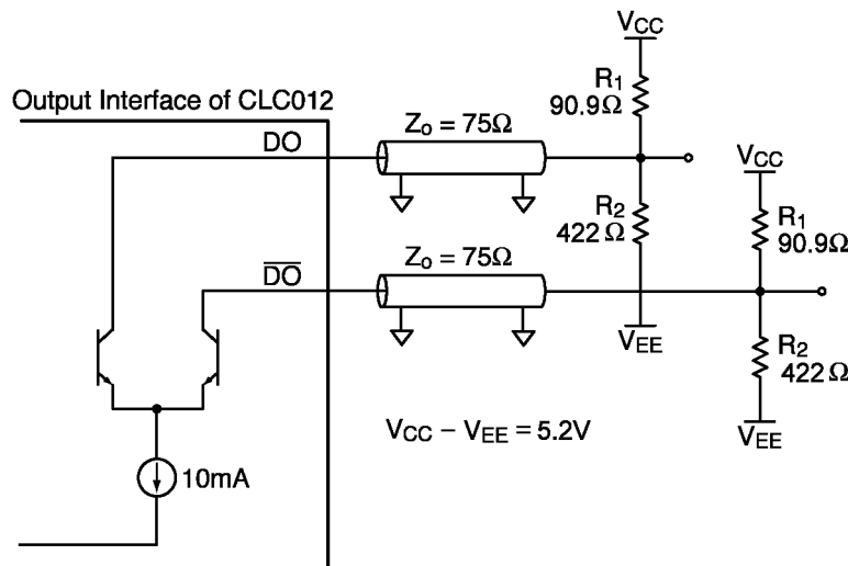
Figure 8. Alternative Load Terminated Output Interface
