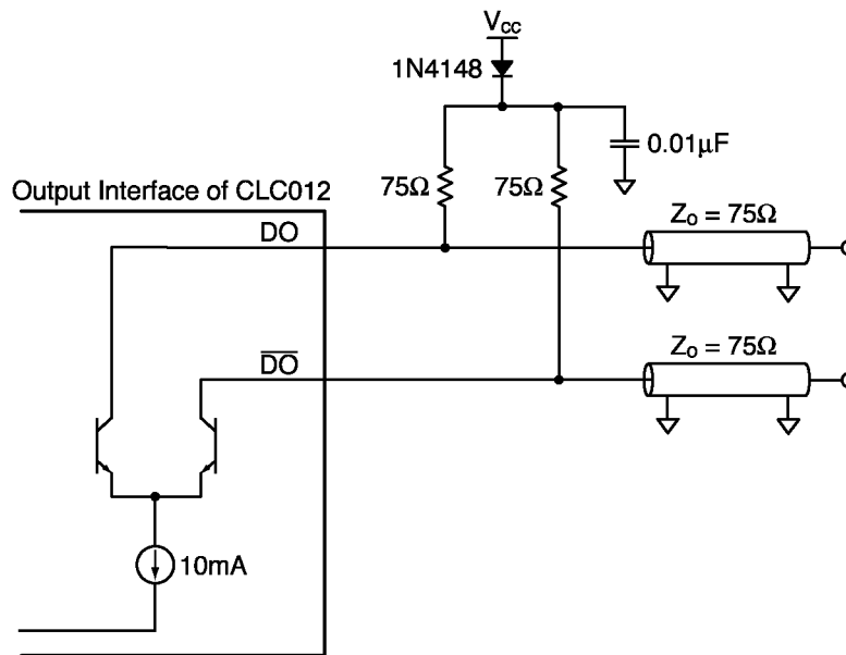
Figure 7. Differential Source Terminated Output Interface
