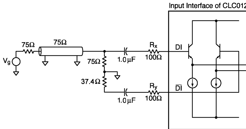
Figure 4. Single-Ended 75Ω Cable Input Interface
