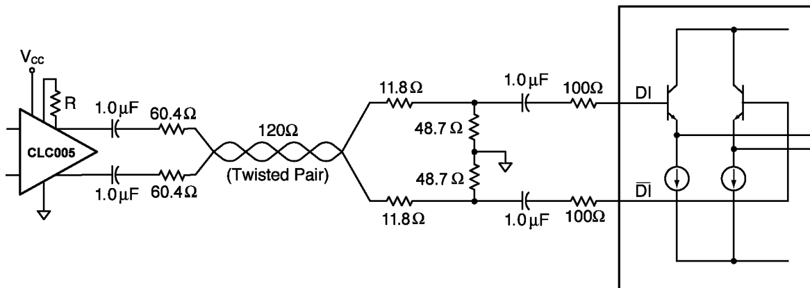
Figure 14. Twisted Pair Equalization
