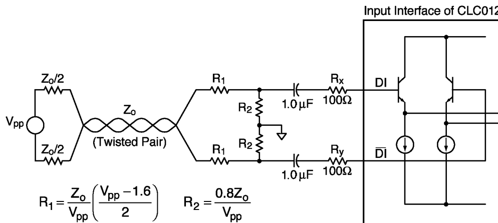
Figure 5. Twisted Pair Input Interface
