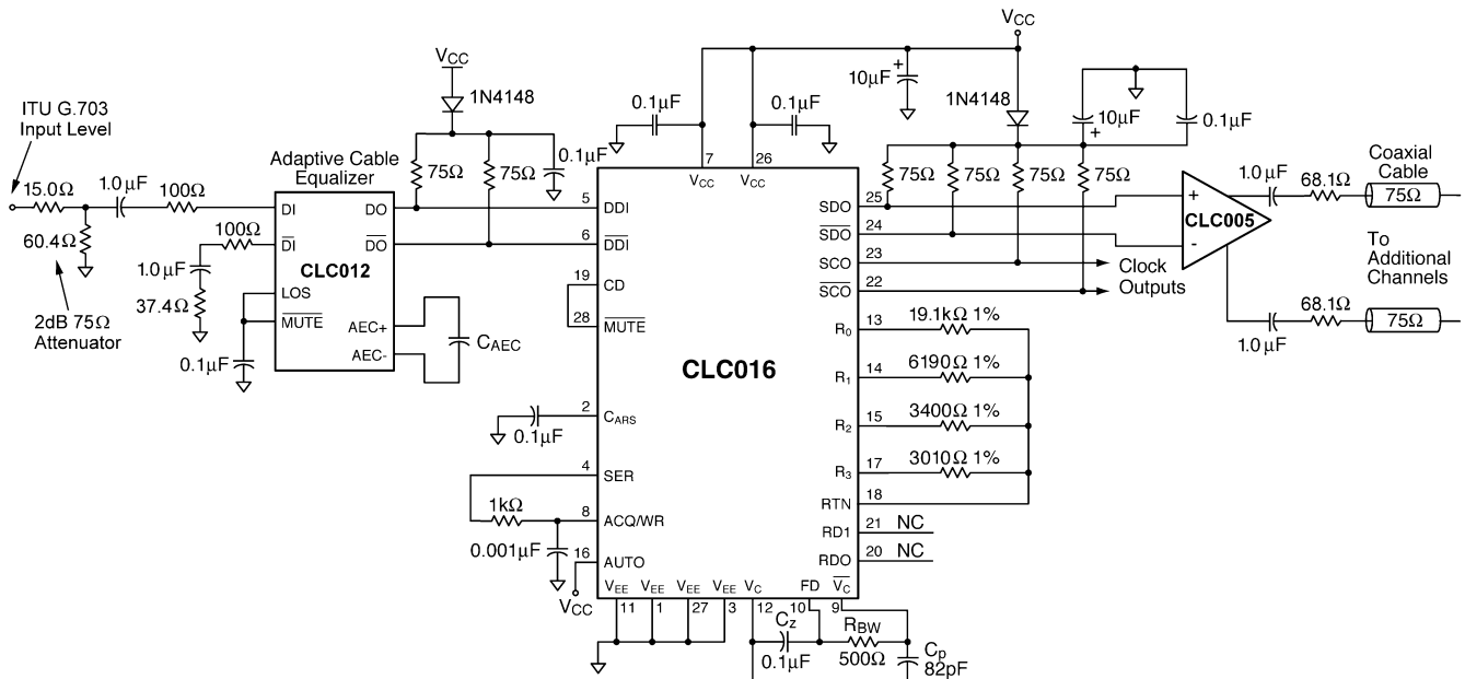
Figure 12. Typical Repeater Design
