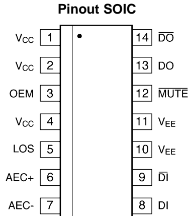
Figure 1. 14-Pin SOIC
