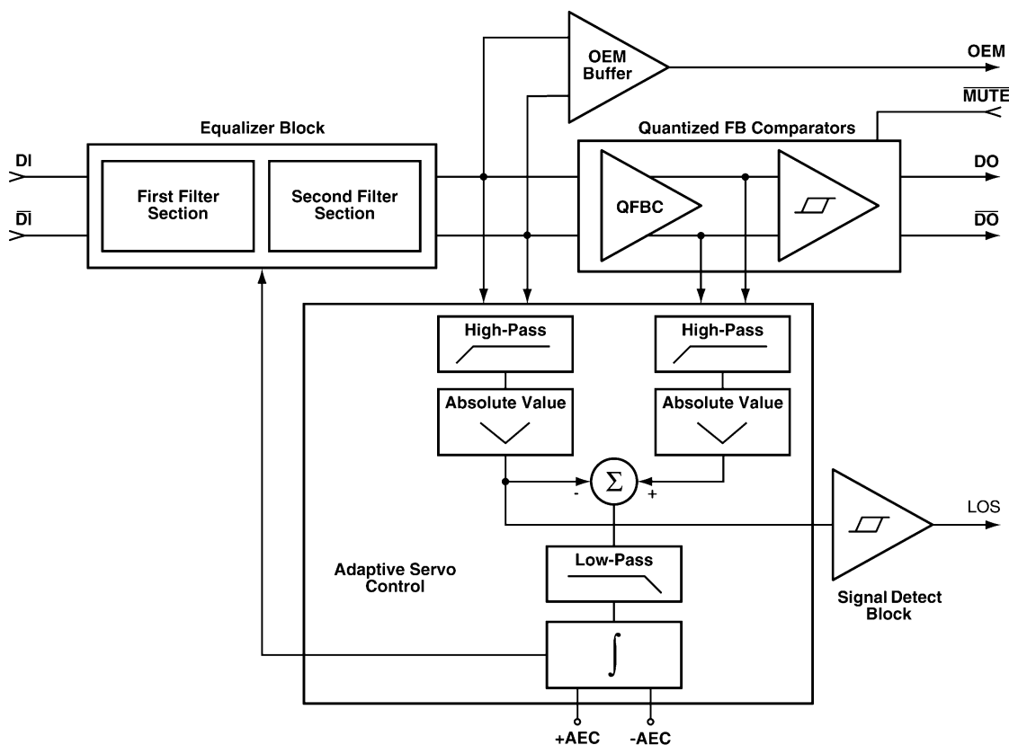
Figure 3. CLC012 Block Diagram
