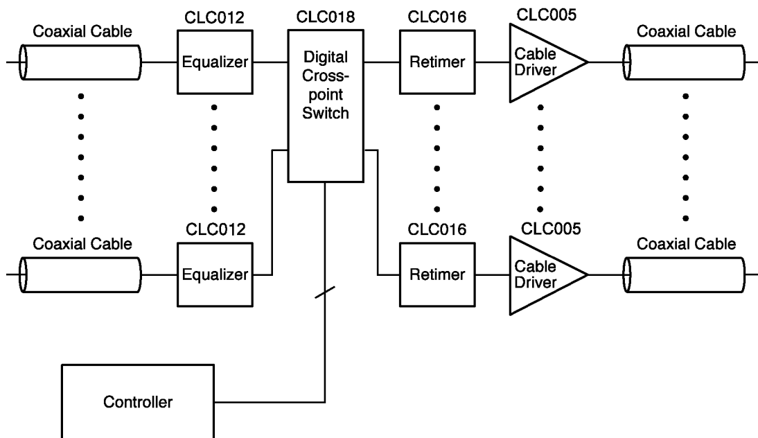
Figure 13. Data Routing Block Diagram
