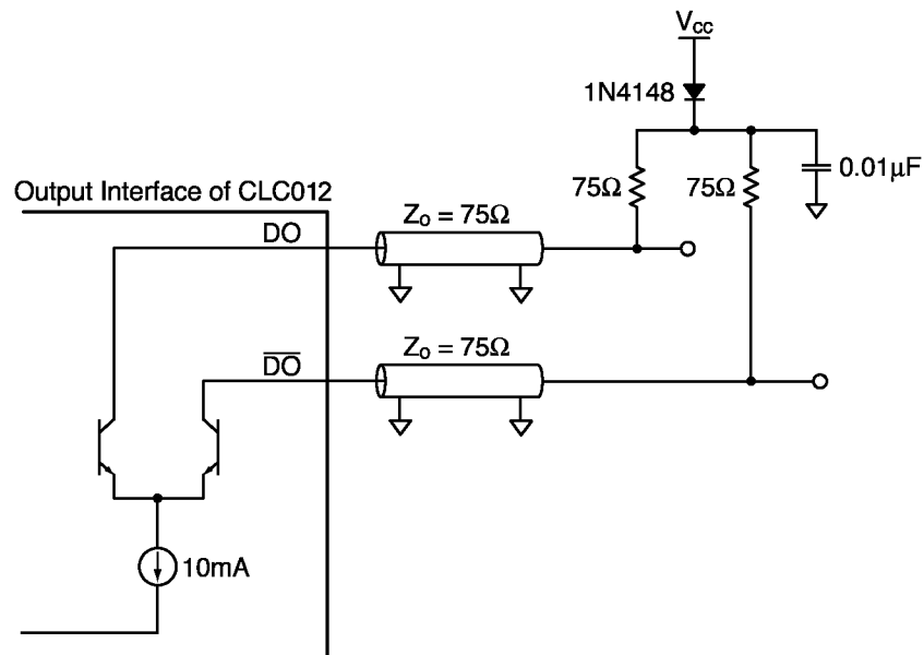
Figure 6. Differential Load Terminated Output Interface
