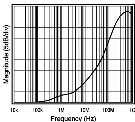
Figure 11. Maximum Equalization Response
