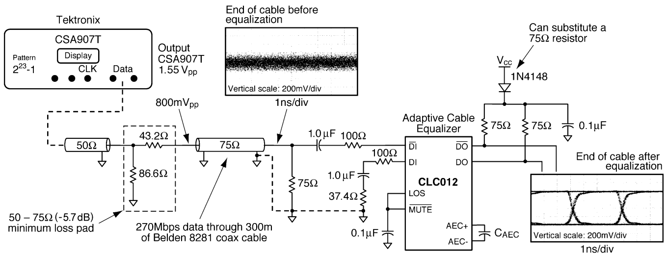
Figure 16. Typical Measurement Setup
