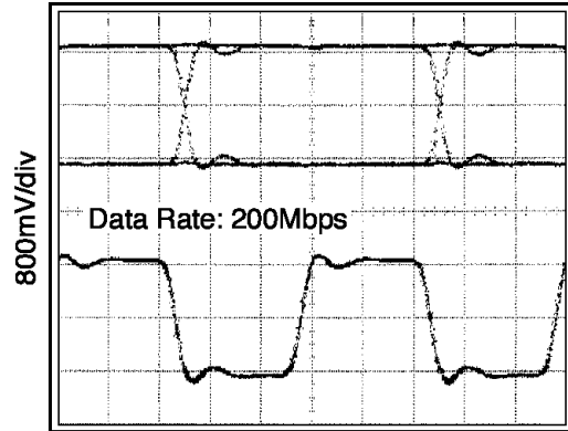
1ns/div Figure 5.
