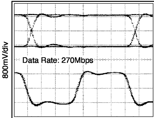
500ps/div Figure 6.
