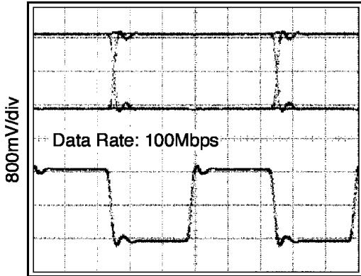
2ns/div Figure 4.
