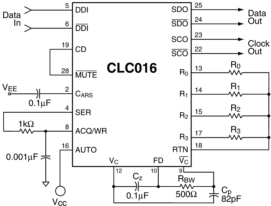
Figure 1. Four-Rate Clock and Data Recovery with Automatic Rate Selection - PLCC Package shown
