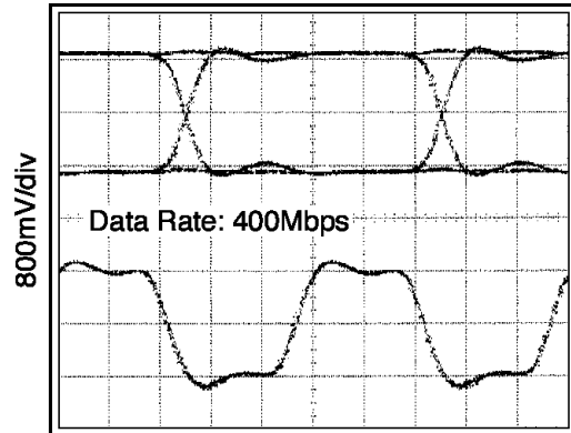
500ps/div Figure 7.
