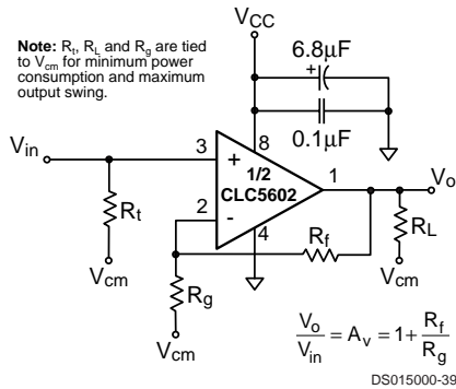
FIGURE 1. Non-Inverting Configuration
