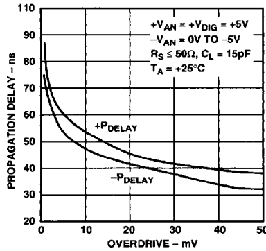
Figure 3. CMP402 Propagation Delay vs. Overdrive
