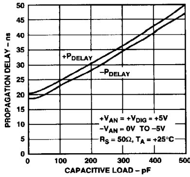
Figure 12. CMP401 Propagation Delay vs. Capacitive Load
