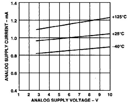
Figure 25. CMP402 Analog Supply Current vs. Analog Supply Voltage
