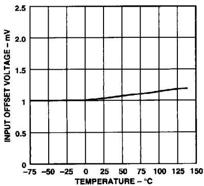
Figure 17. CMP401/CMP402 Input Offset Voltage vs. Temperature
