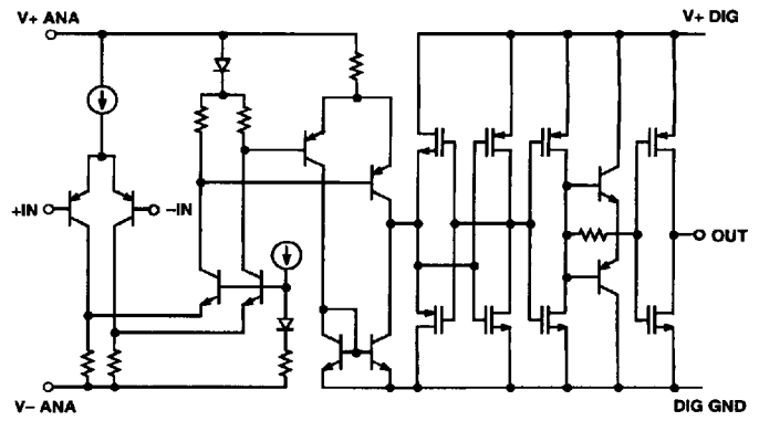
Figure 1. Simplified Schematic
