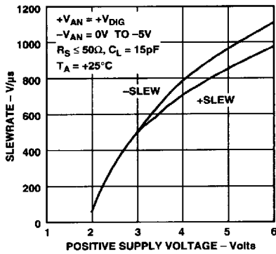
Figure 14. CMP401/CMP402 Slew Rate vs. Positive Supply Voltage
