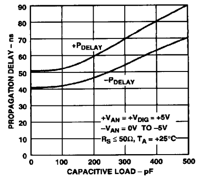
Figure 13. CMP402 Propagation Delay vs. Capacitive Load
