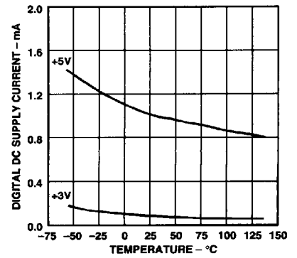
Figure 19. CMP402 Digital Supply Current vs. Temperature
