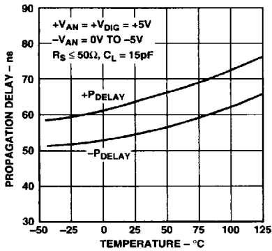
Figure 5. CMP402 Propagation Delay vs. Temperature - 5 mV OD
