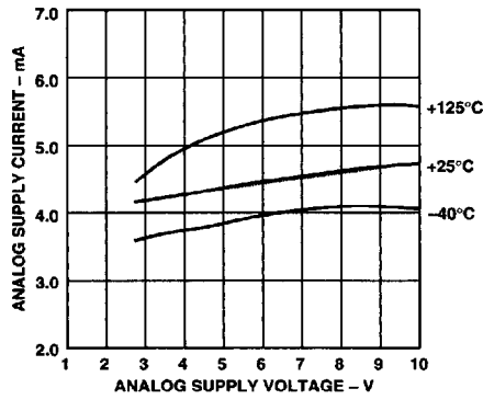
Figure 24. CMP401 Analog Supply Current vs. Analog Supply Voltage
