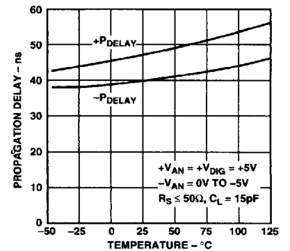
Figure 7. CMP402 Propagation Delay vs. Temperature - 20 mV OD
