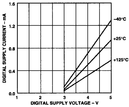
Figure 20. CMP401 Digital Supply Current vs. Digital Supply Voltage
