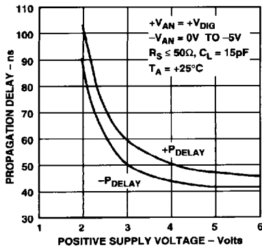
Figure 11. CMP402 Propagation Delay vs. Supply Voltage – 20 mV OD
