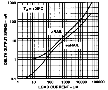
Figure 16. CMP401/CMP402 Delta Output Swing from Power Supplies vs. Load Current
