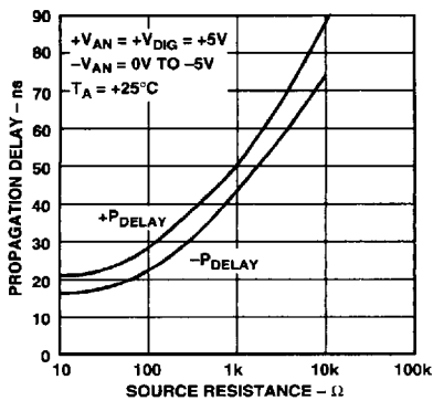
Figure 8. CMP401 Propagation Delay vs. Source Resistance - 20 mV OD
