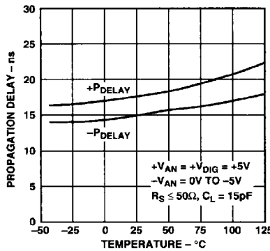
Figure 6. CMP401 Propagation Delay vs. Temperature - 20 mV OD
