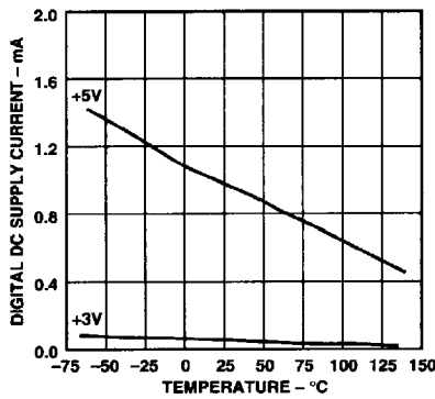
Figure 18. CMP401 Digital Supply Current vs. Temperature
