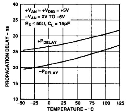
Figure 4. CMP401 Propagation Delay vs. Temperature - 5 mV OD
