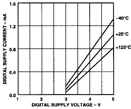
Figure 21. CMP402 Digital Supply Current vs. Digital Supply Voltage
