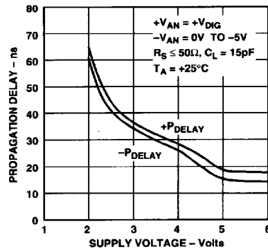
Figure 15. CMP401 Propagation Delay vs. Supply Voltage
