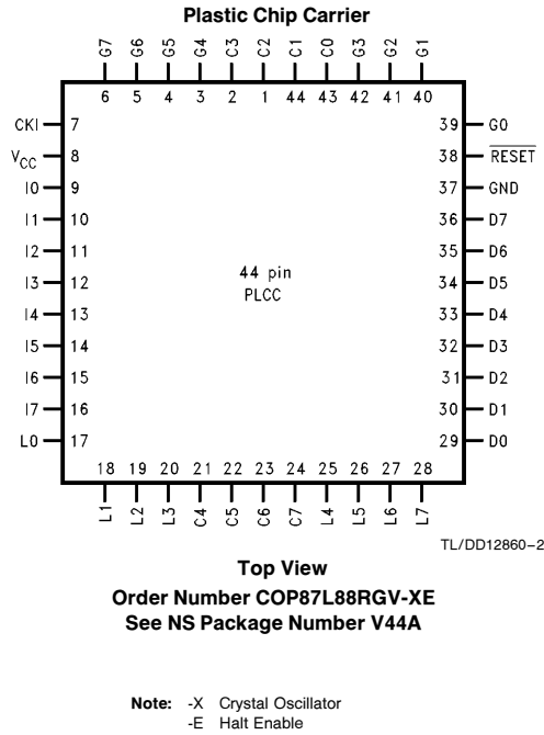
FIGURE 2. Connection Diagrams
