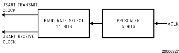
FIGURE 23. USART BAUD Clock Generation
