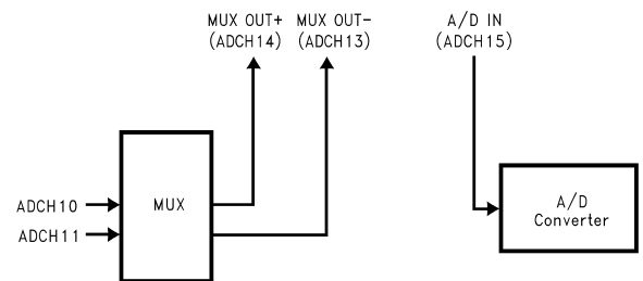
FIGURE 27. A/D with Differential Mux Output Feature Enabled
