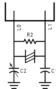
Low Speed Oscillator
