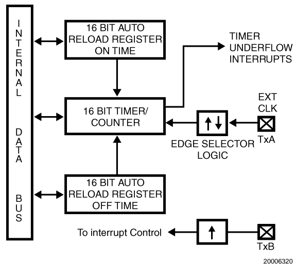
FIGURE 16. Timer in External Event Counter Mode
