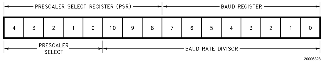
FIGURE 24. USART BAUD Clock Divisor Registers
