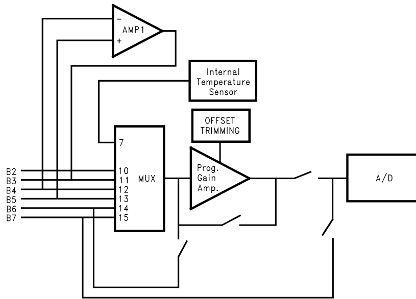
FIGURE 25. Simplified A/D Converter Block Diagram
