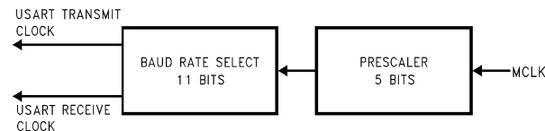
FIGURE 24. USART BAUD Clock Generation
