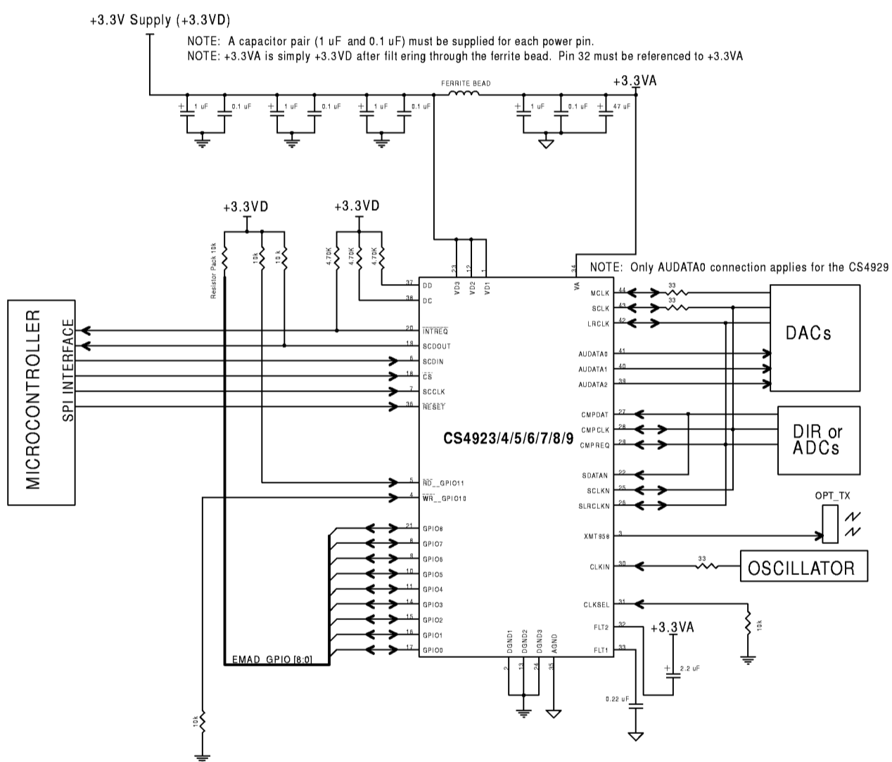
Figure 15. SPI Control
